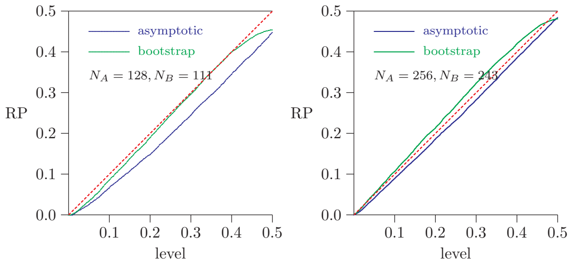
Figure 5. P value plots for larger sample sizes
